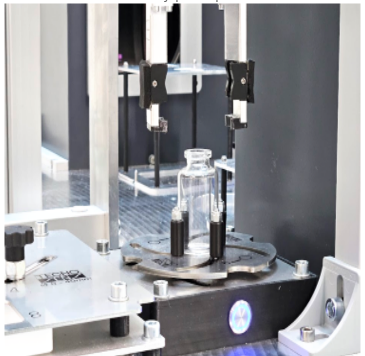
Self-centering pick-up
