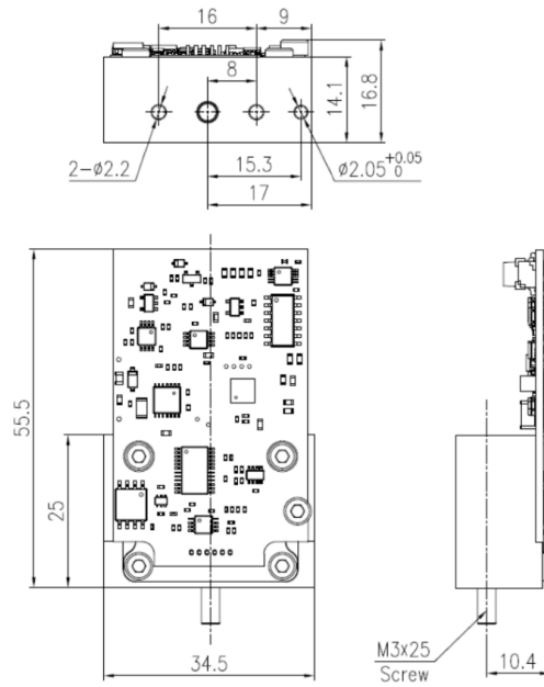
Figure 3.2: TSF5001, full scale of 200 sccm manifold mechanical dimensions.
