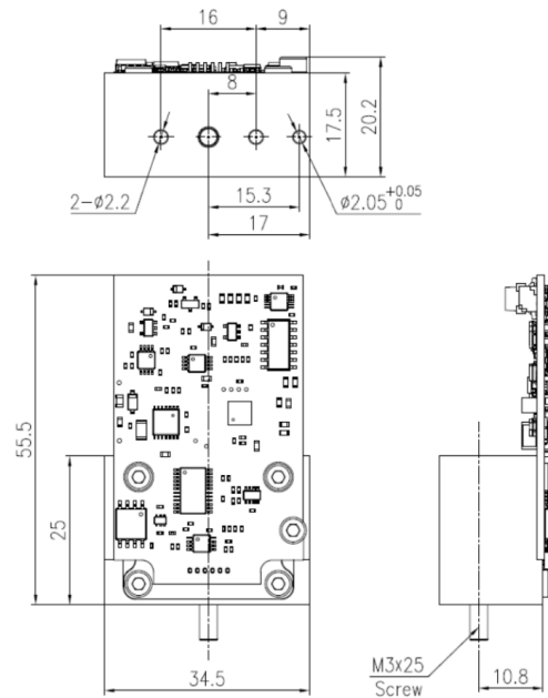
Figure 3.3: TSF5001, full scale of 500, 1k, 2k and 4k sccm (up to 5k sccm / 5 SLPM) manifold mechanical dimensions.
