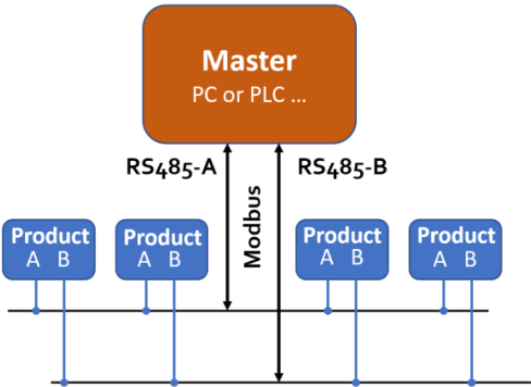
Figure 5.1: RS485 hardware
