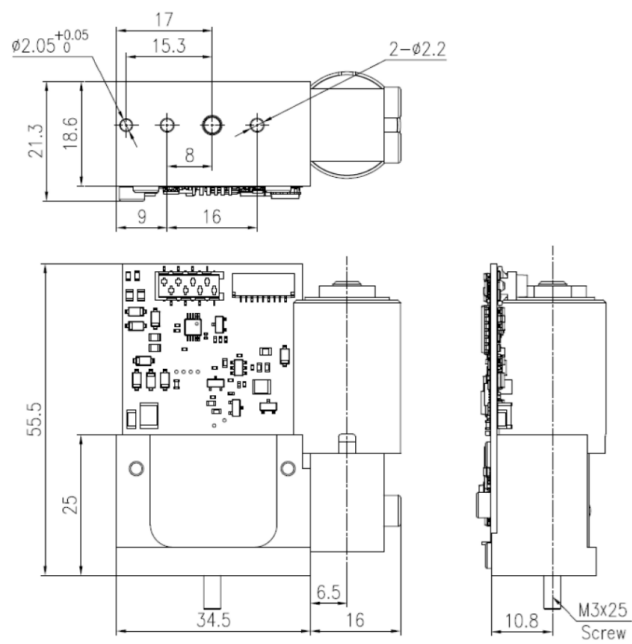
Figure 3.4: TSFC5001 (up to 5k sccm / 5 SLPM) manifold mechanical dimensions.
